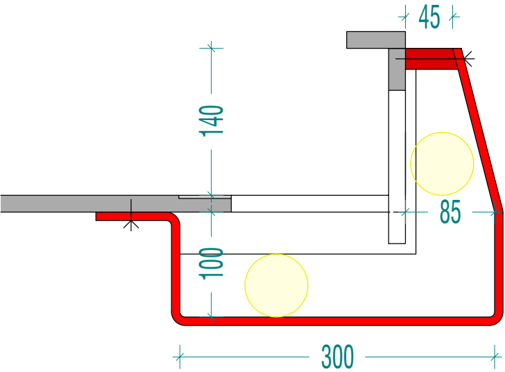
section | 1:5
